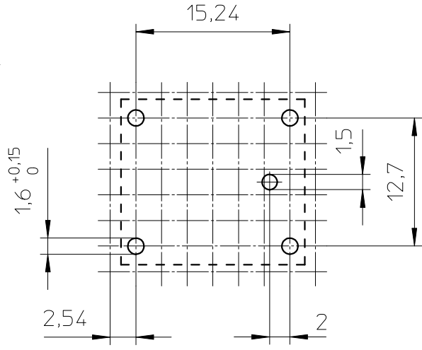
HOLE PATTERN:
